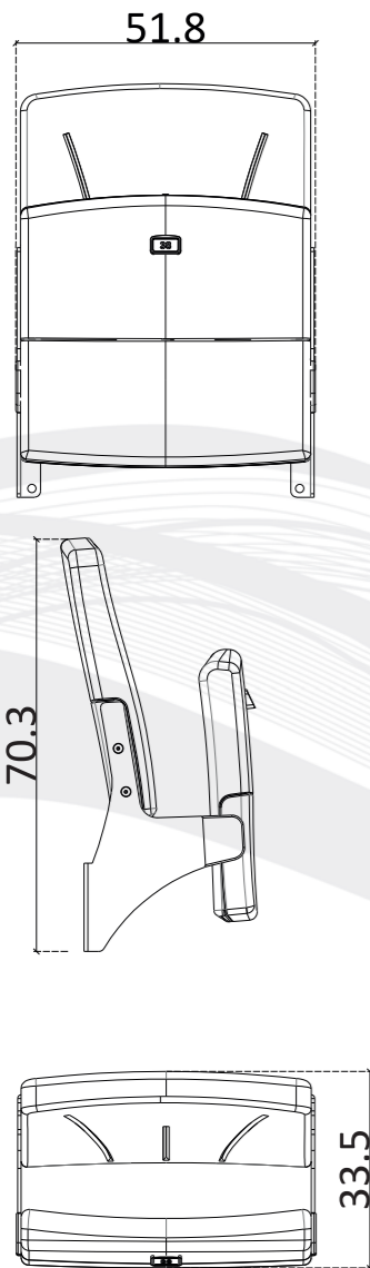
ROYAL-101 STANDARD
