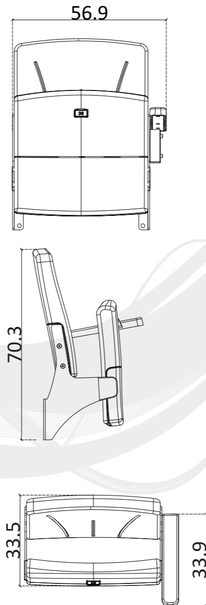
ROYAL-102 ARMREST
